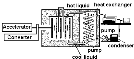
Fig. 3. Accelerator Driven Reactor
