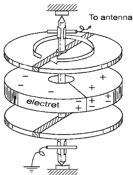
Figure 4. Electrostatic Motor Model
